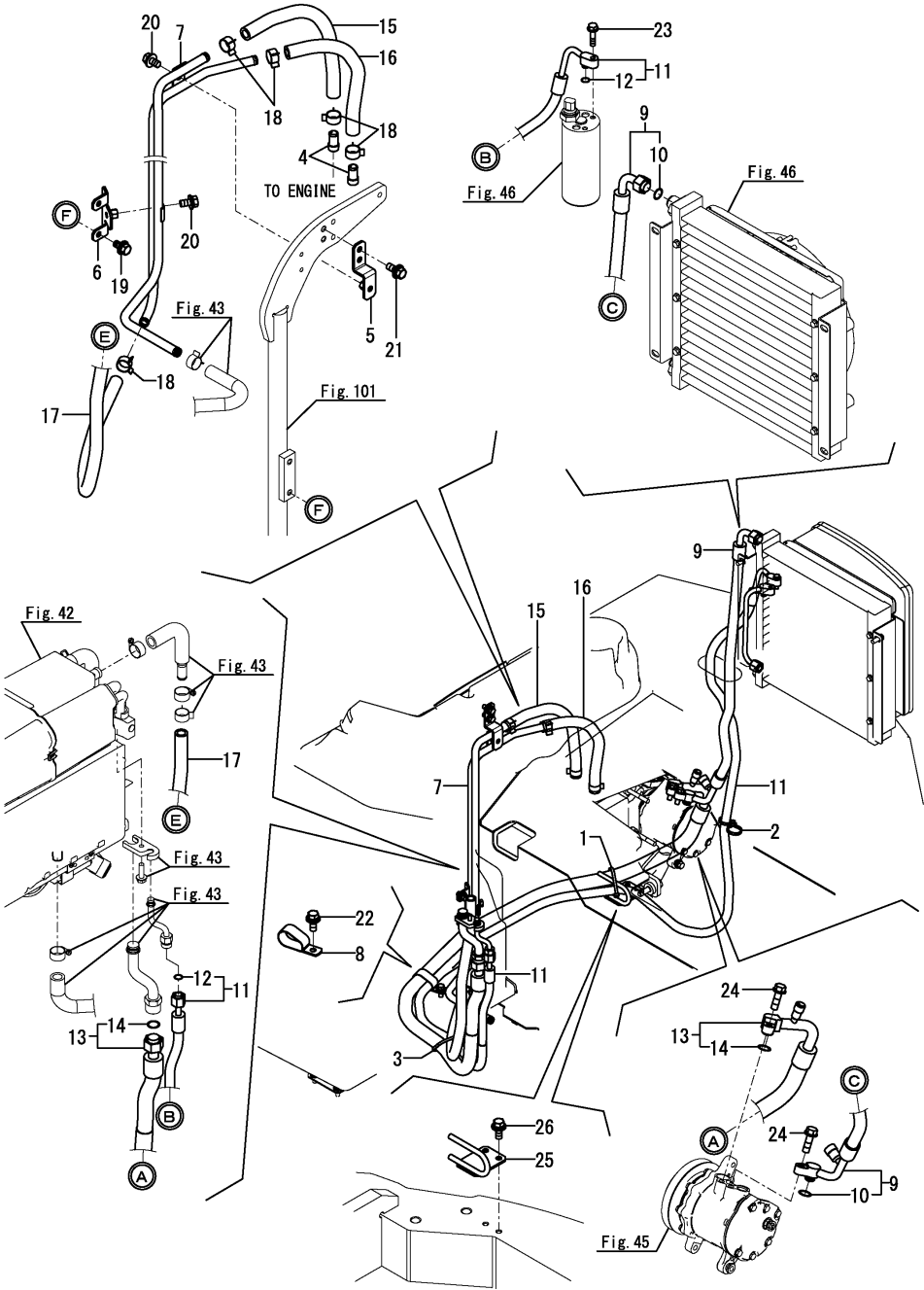
Fig.44. AIR CONDITIONER(PIPING)
