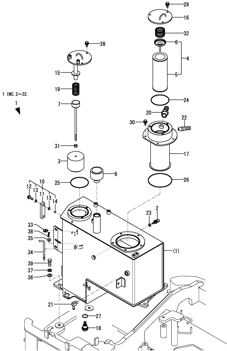
Fig.160. HYD. OIL TANK
