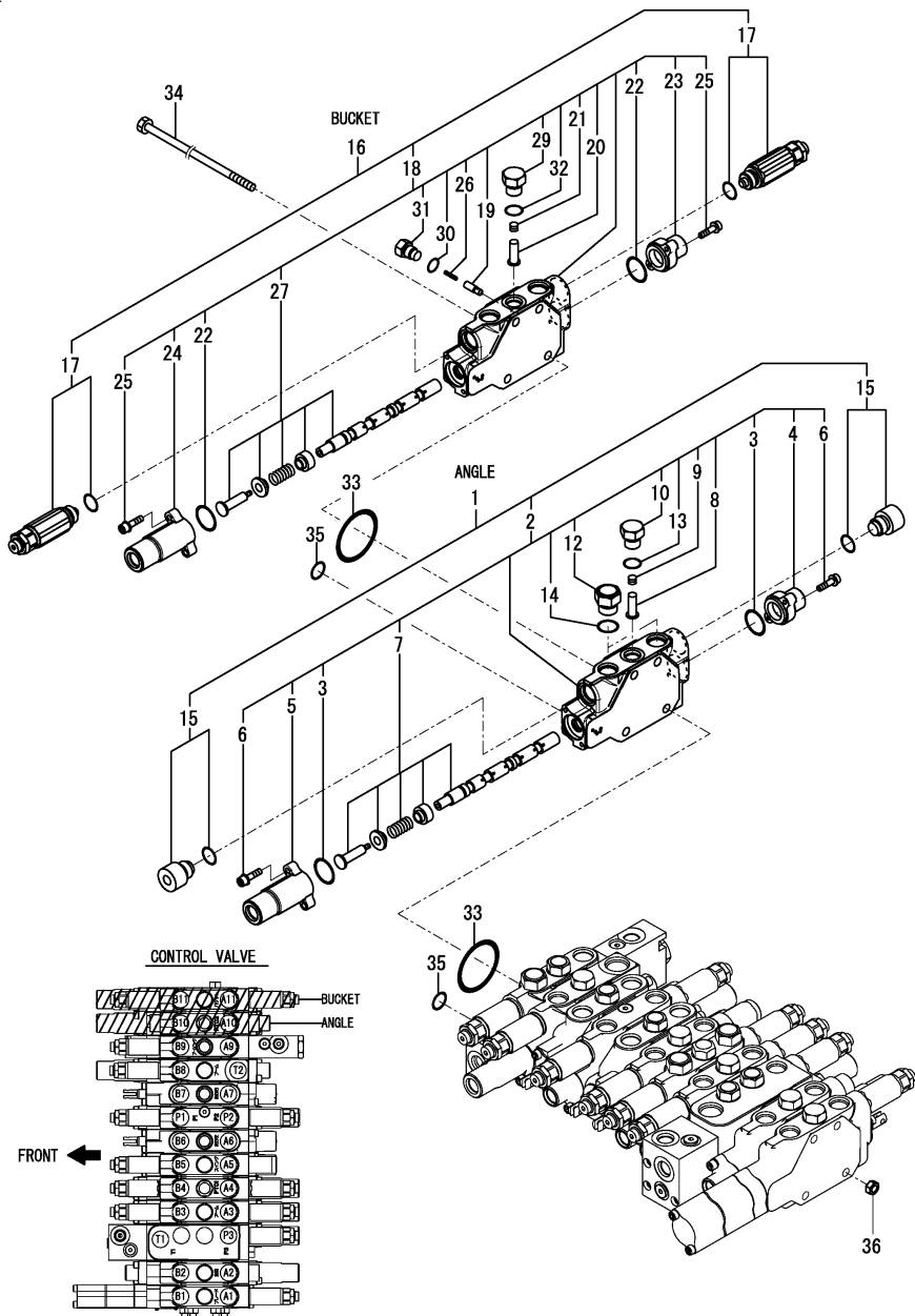
Fig.145. CONTROL VALVE(2/8)(ANGLE BLADE SPEC.)
