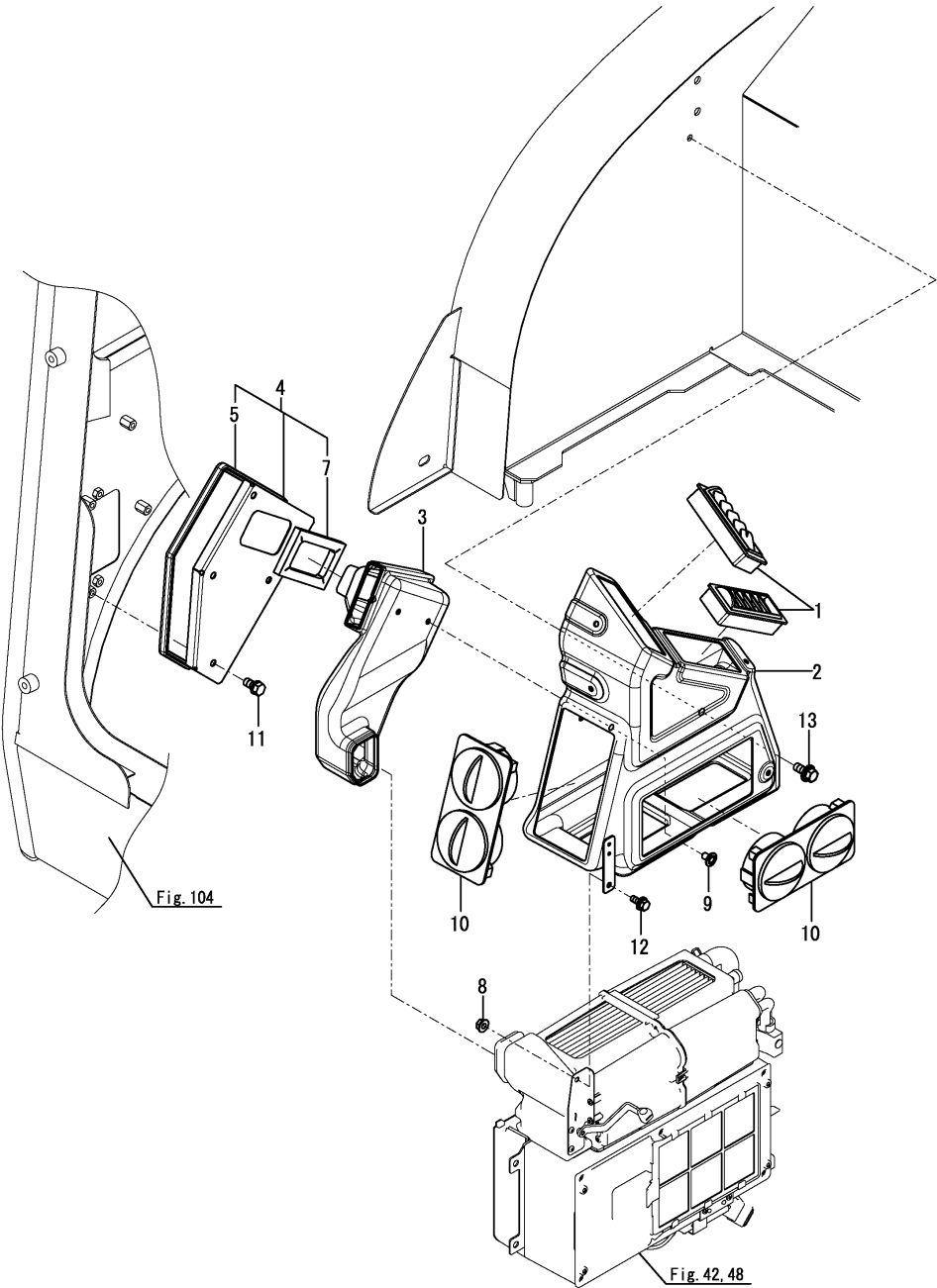
Fig.51. DUCT(AIR CONDITIONER & HEATER)
