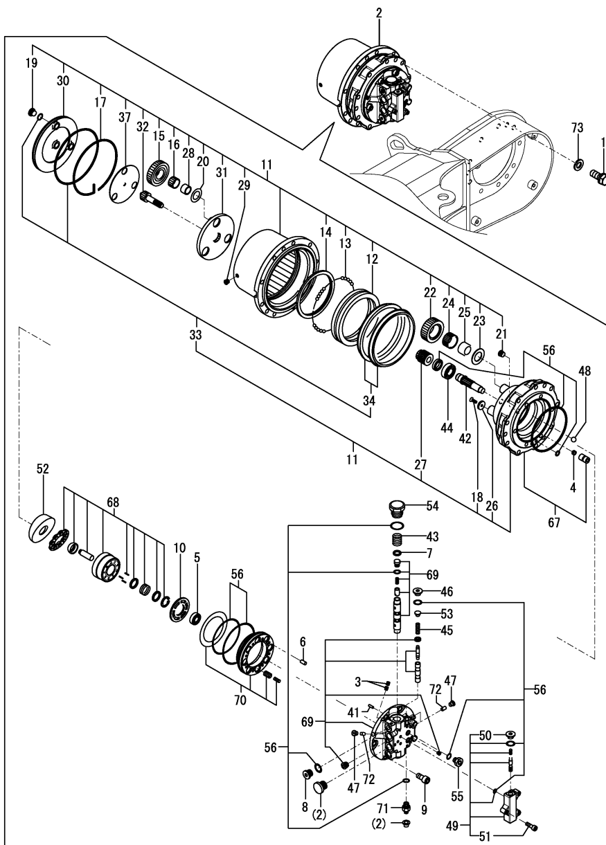
Fig.131. TRAVEL MOTOR
