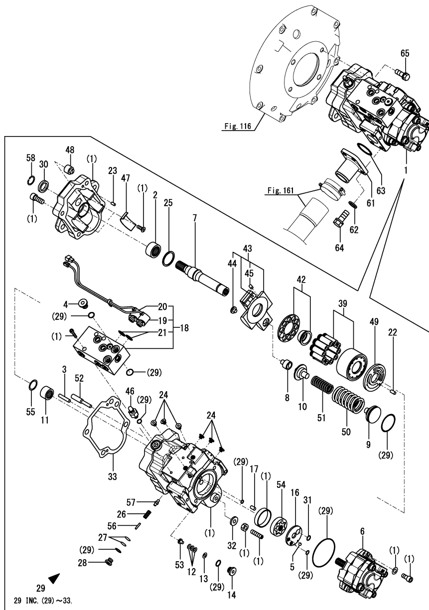
Fig.117. HYDRAULIC PUMP
