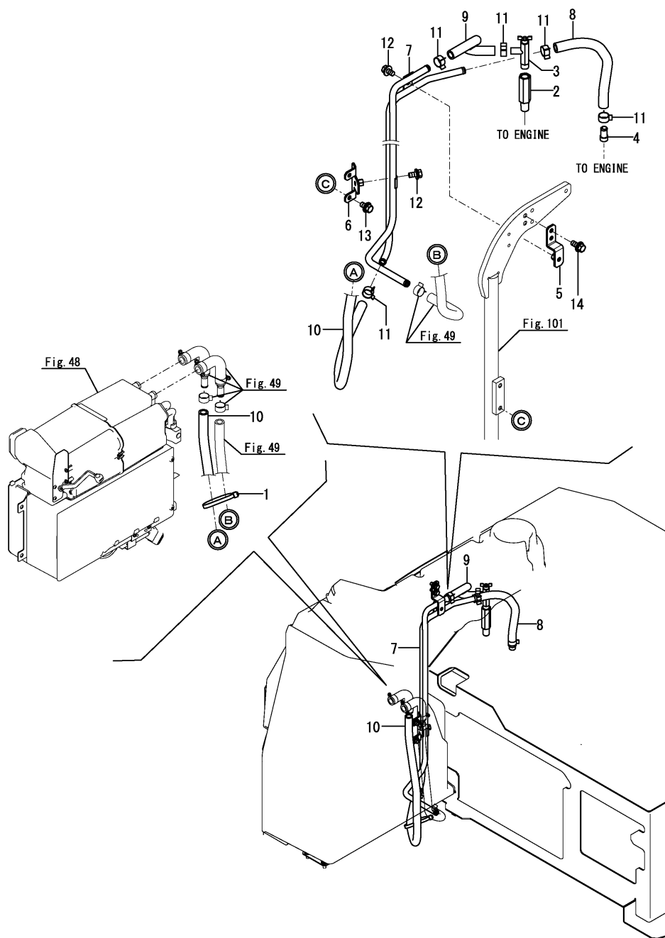
Fig.50. HEATER(PIPING)
