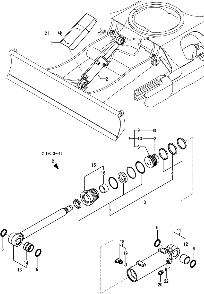
Fig.126. BLADE CYLINDER
