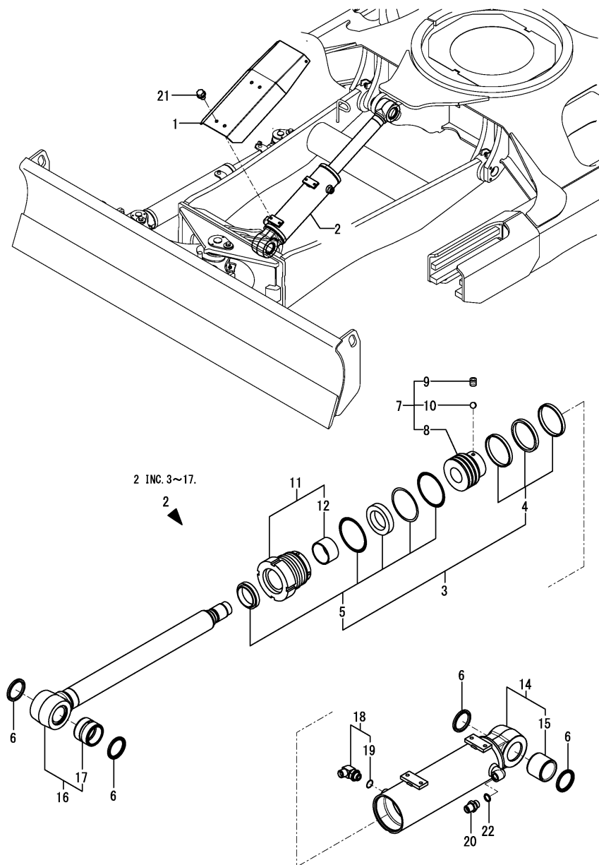
Fig.128. BLADE CYLINDER(ANGLE BLADE SPEC.)
