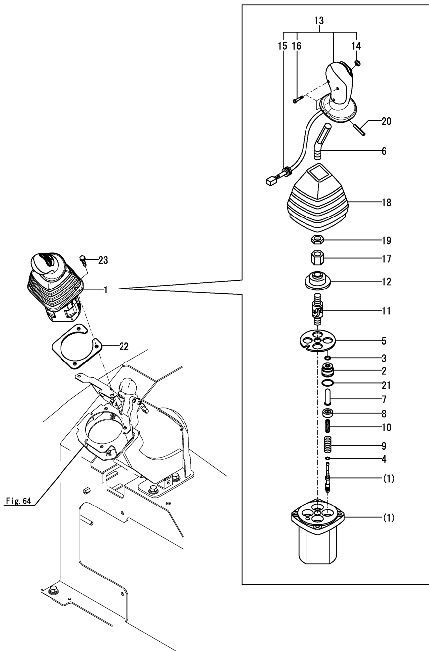
Fig.152. REMOTE CONTROL VALVE(RIGHT)
