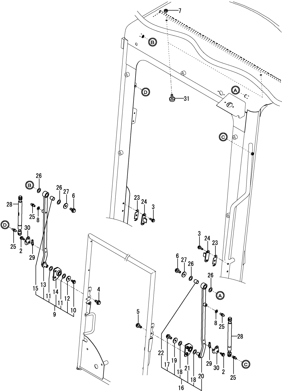
Fig.107. CABIN(FRONT WINDOW)(1)
