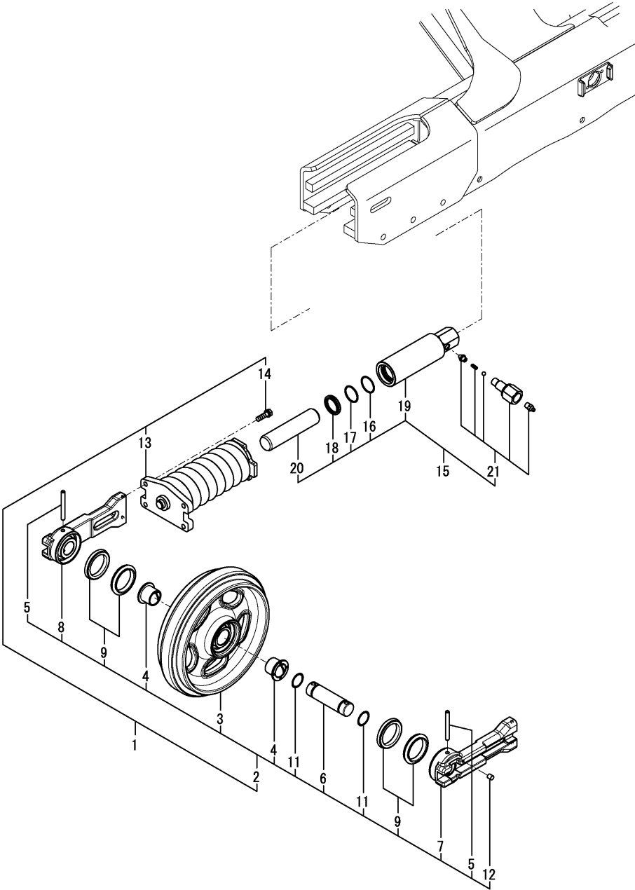
Fig.53. IDLER & ADJUST
