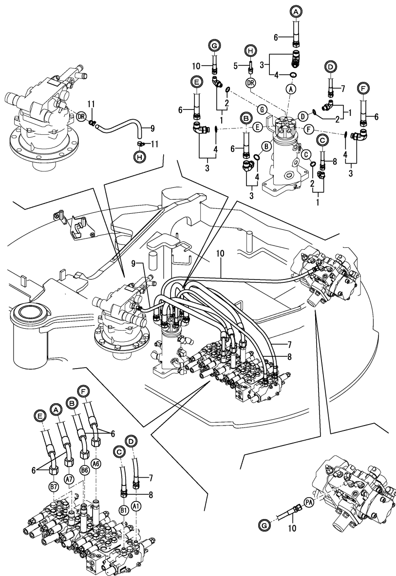
Fig.170. CONTROL VALVE - SWIVEL JOINT
