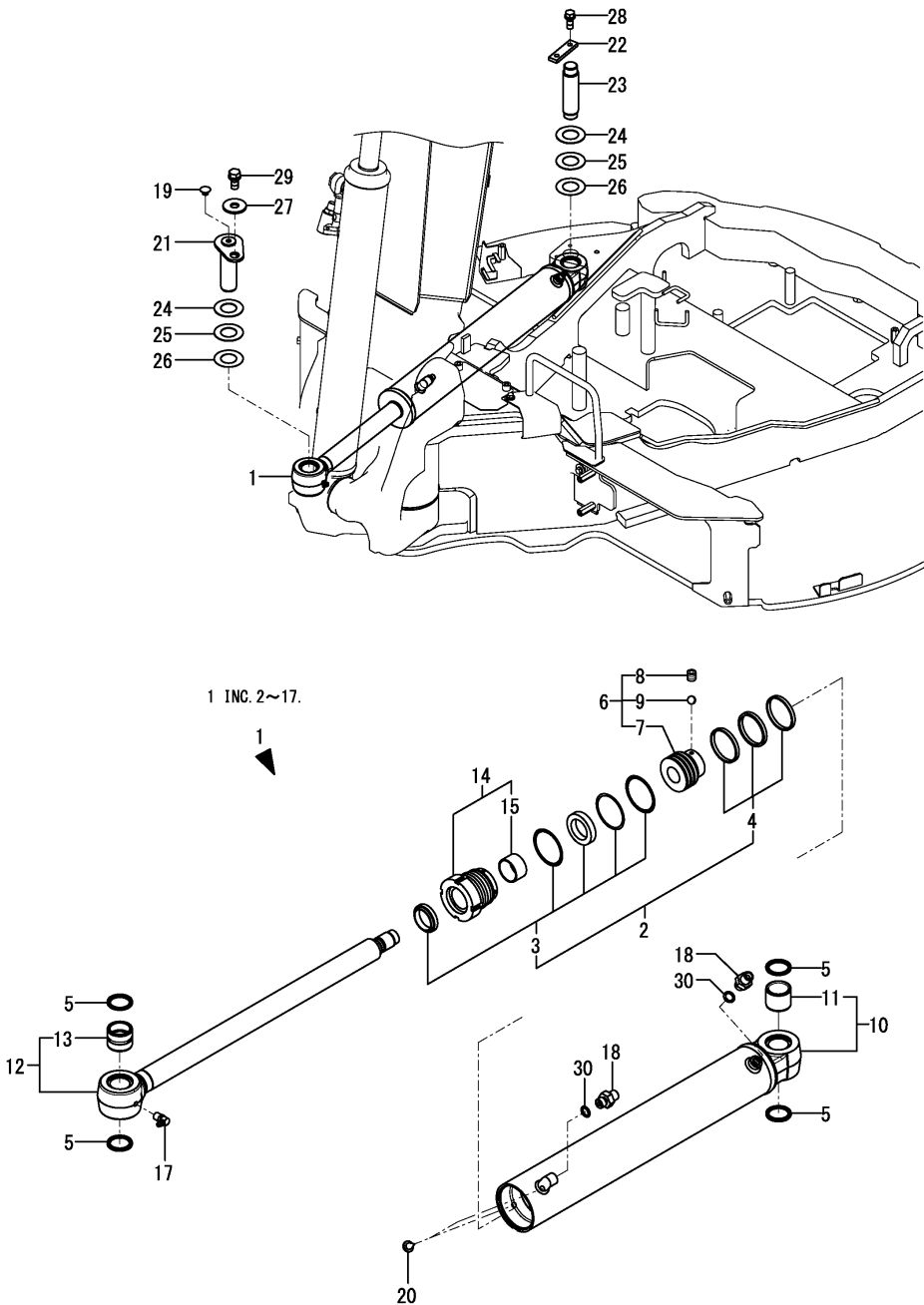
Fig.125. SWING CYLINDER
