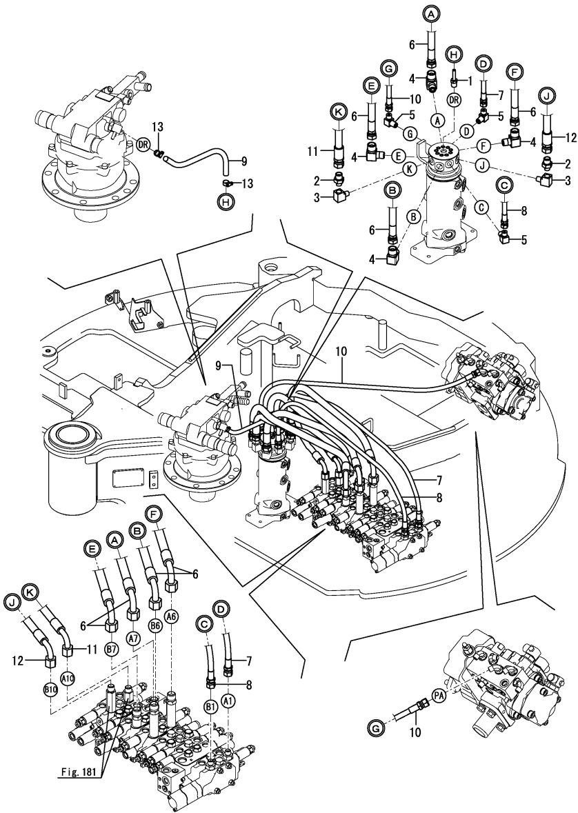
Fig.171. CONTROL VALVE - SWIVEL JOINT(ANGLE BLADE SPEC.)
