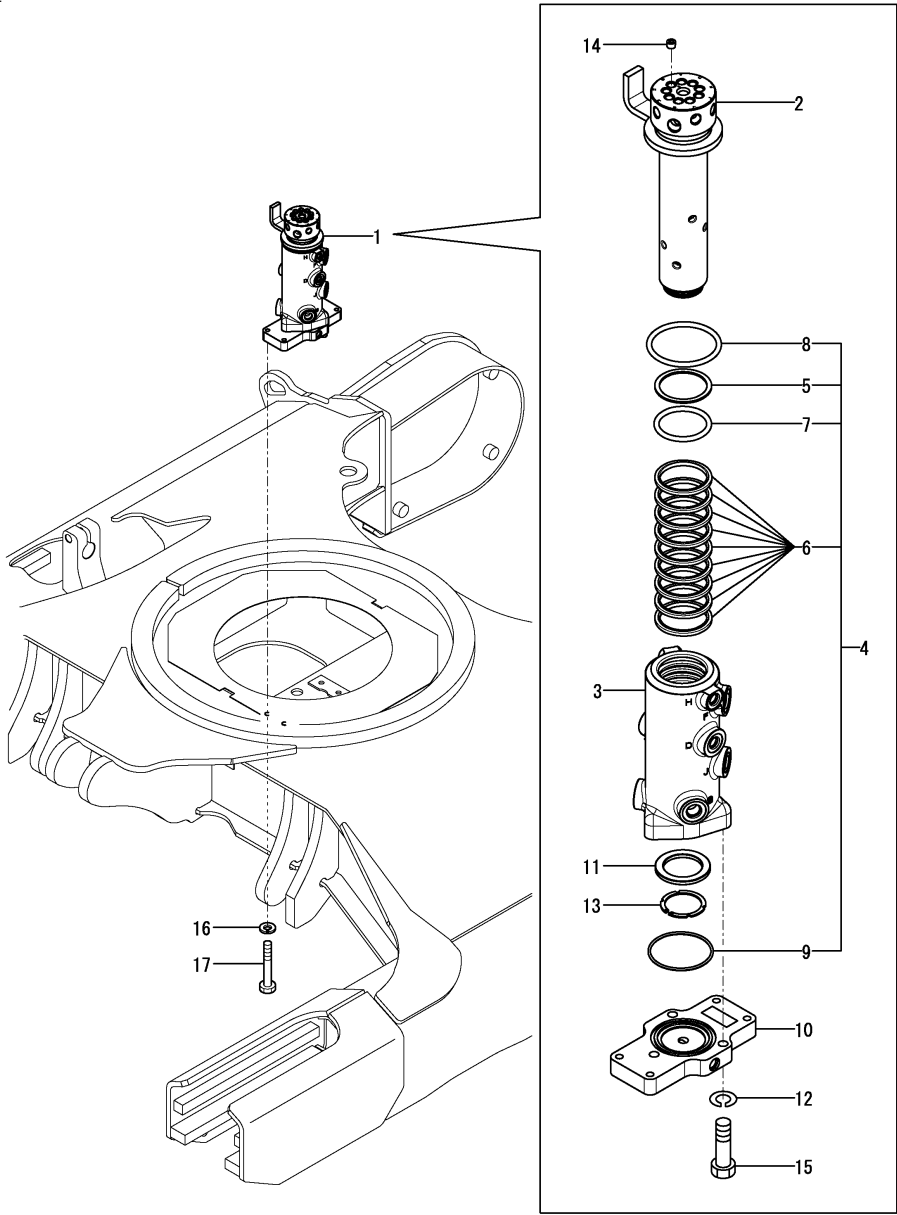
Fig.135. SWIVEL JOINT(ANGLE BLADE SPEC.)
