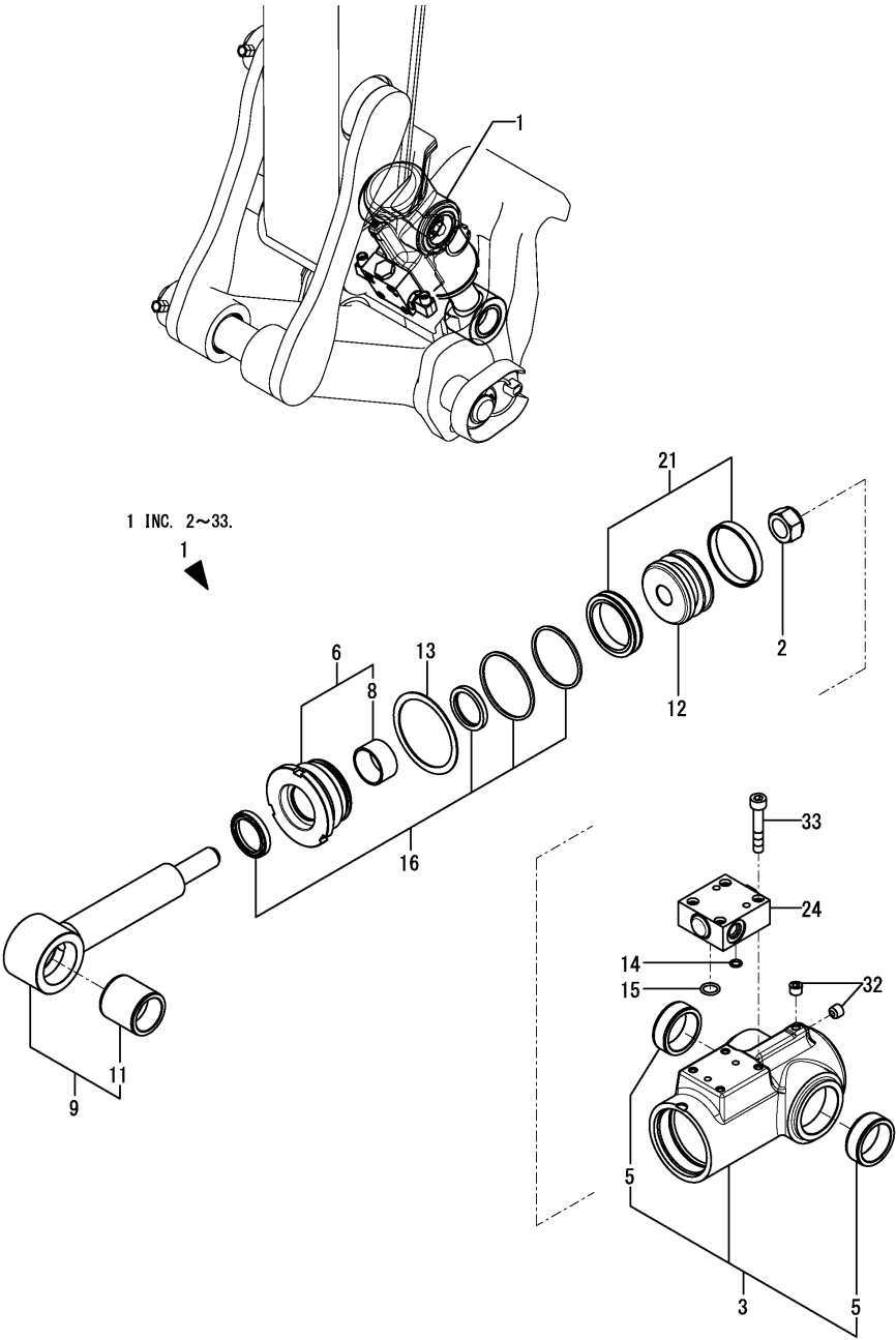
Fig.130. HITCH CYLINDER(QUICK COUPLER)
