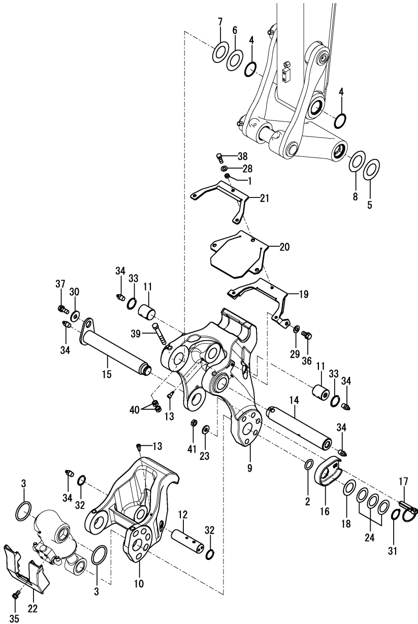
OCK50-M01380 IMPLEMENT Fig.192. QUICK COUPLER(BODY)
