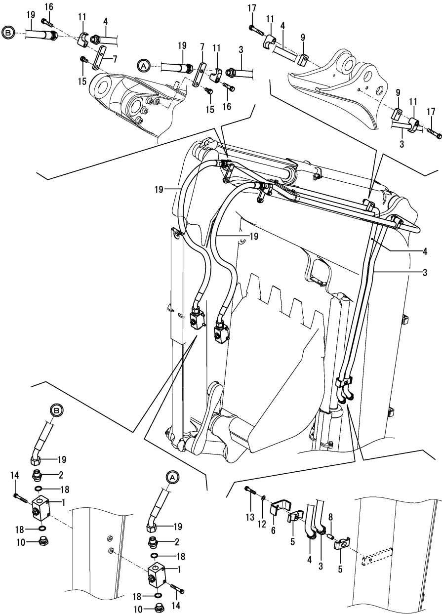
Fig.176. P.T.O.(BOOM - ARM END)
