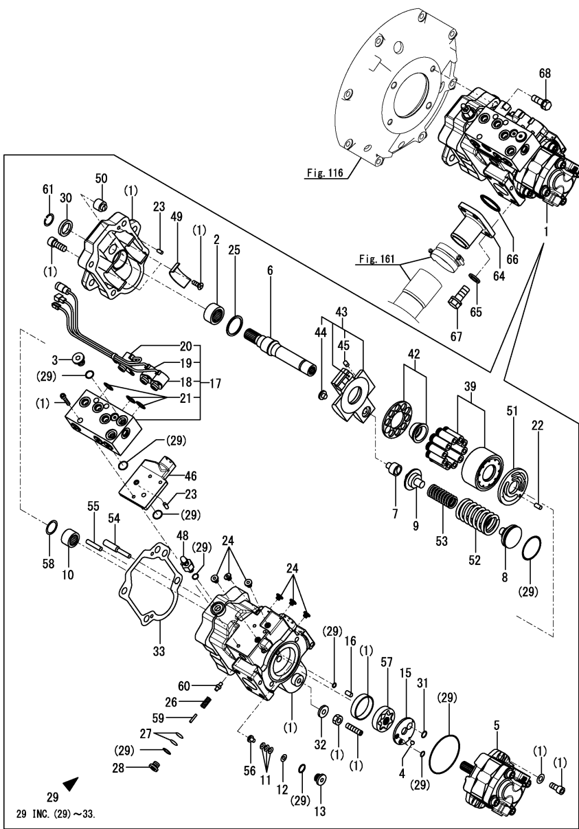
Fig.120. HYDRAULIC PUMP(E.S.S. & QUICK COUPLER SPEC.)
