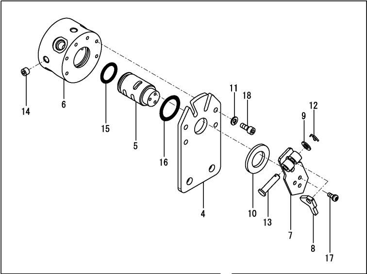
Fig.155. 2-WAY VALVE(ANGLE BLADE SPEC.)
