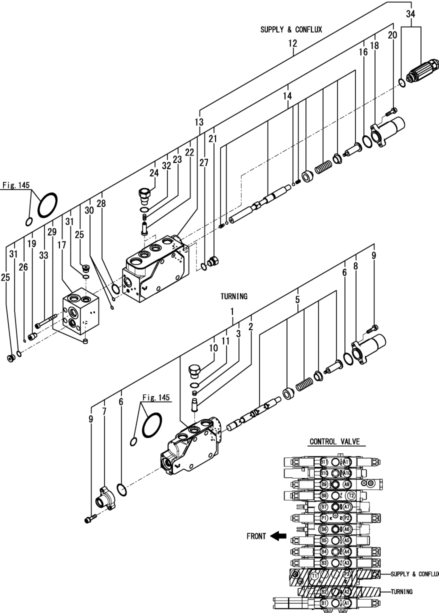
Fig.150. CONTROL VALVE(7/8)(ANGLE BLADE SPEC.)
