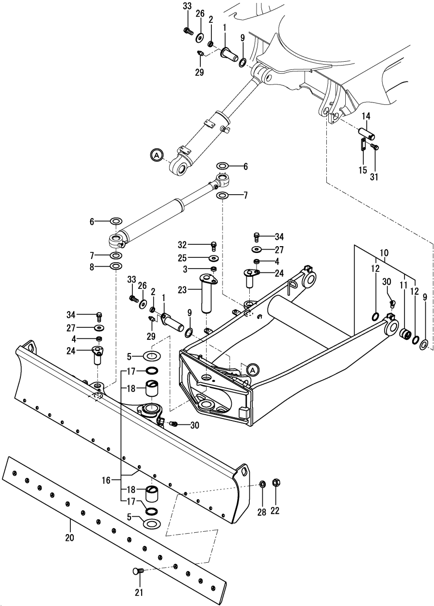
Fig.199. BLADE CYLINDER(ANGLE BLADE SPEC.)
