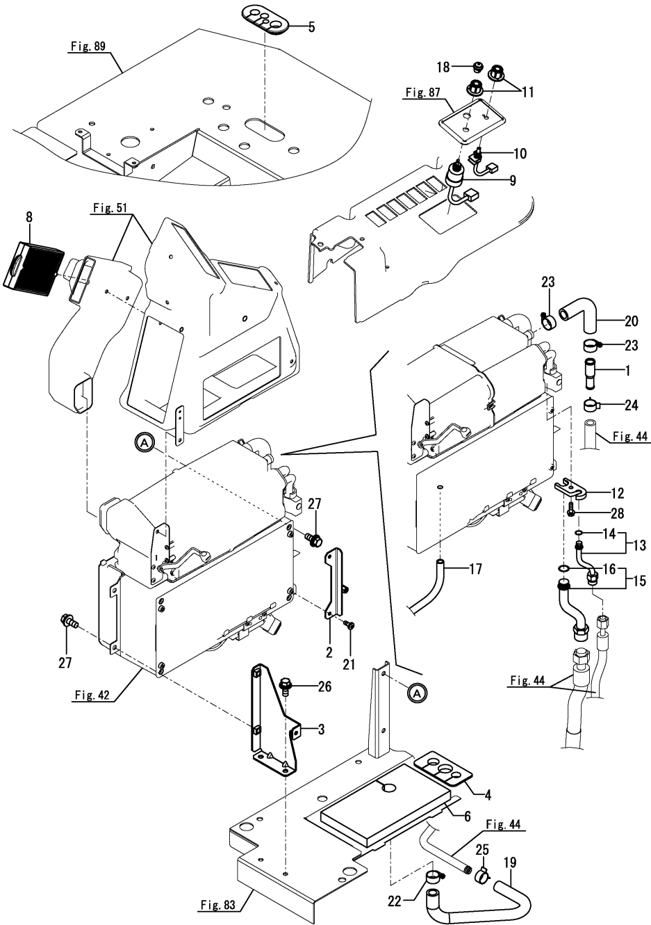
Fig.43. AIR CONDITIONER(ACCESSORY)
