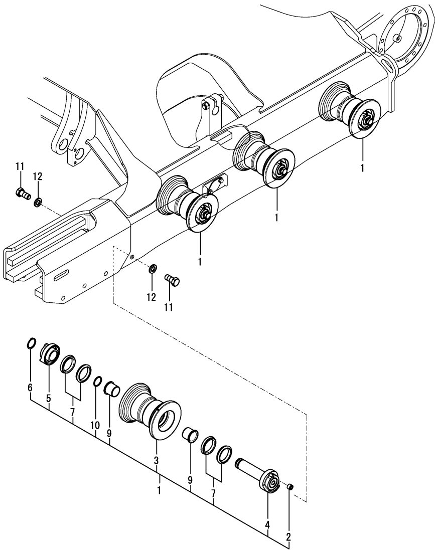
OCK50-M01380 TRAVELING Fig.54. TRACK ROLLER
