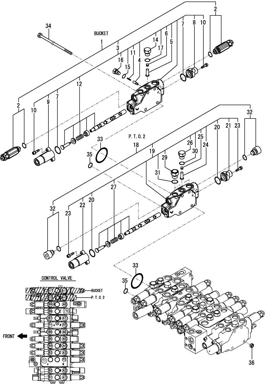
Fig.137. CONTROL VALVE(2/8)
