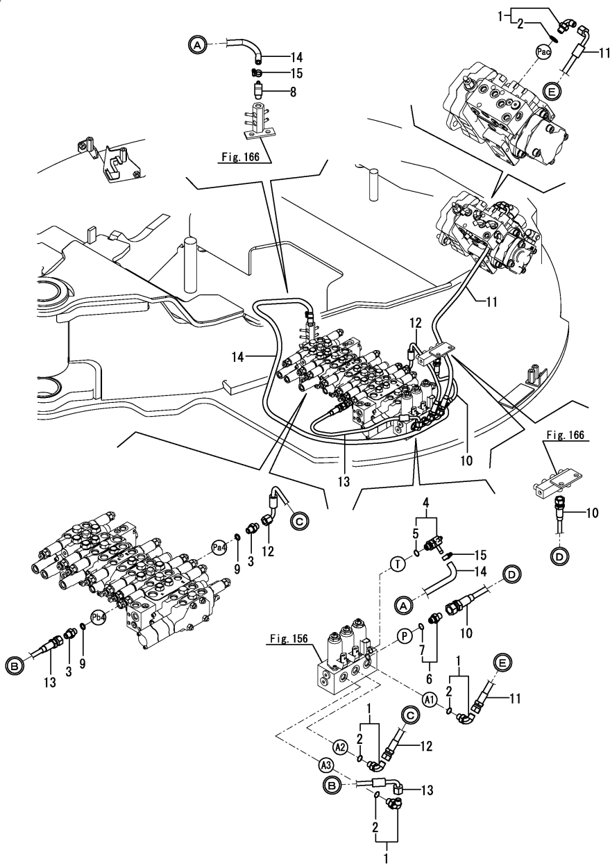
Fig.180. P.T.O.(SOLENOID VALVE & E.S.S.)(ANGLE BLADE SPEC.)
