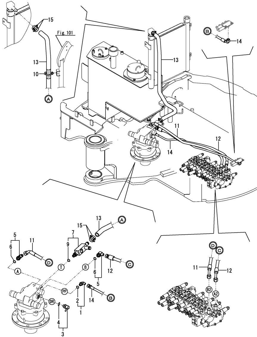
Fig.162. CONTROL VALVE - TURNING MOTOR
