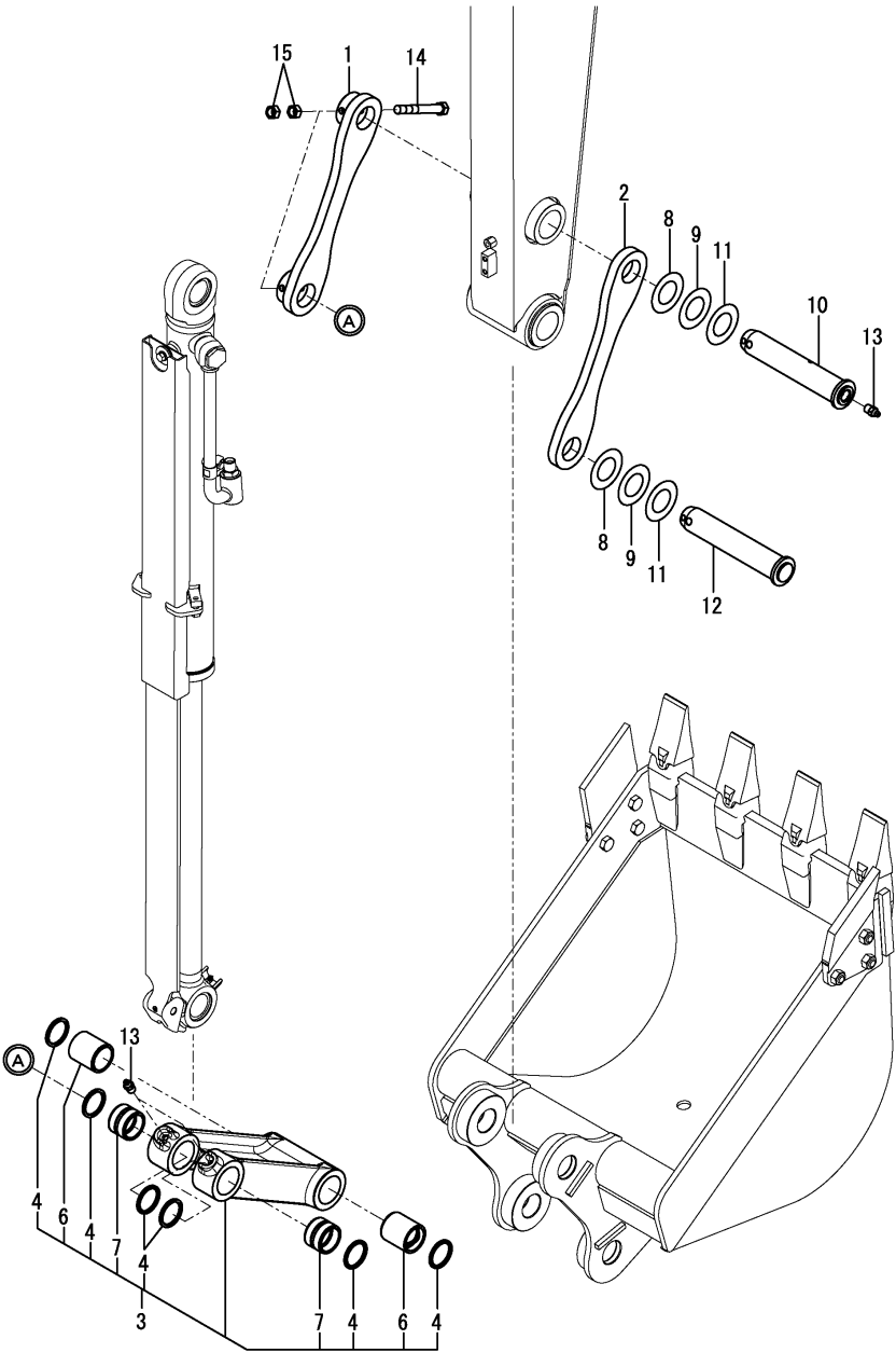
OCK50-M01380 IMPLEMENT Fig.191. BUCKET ARM & LINK
