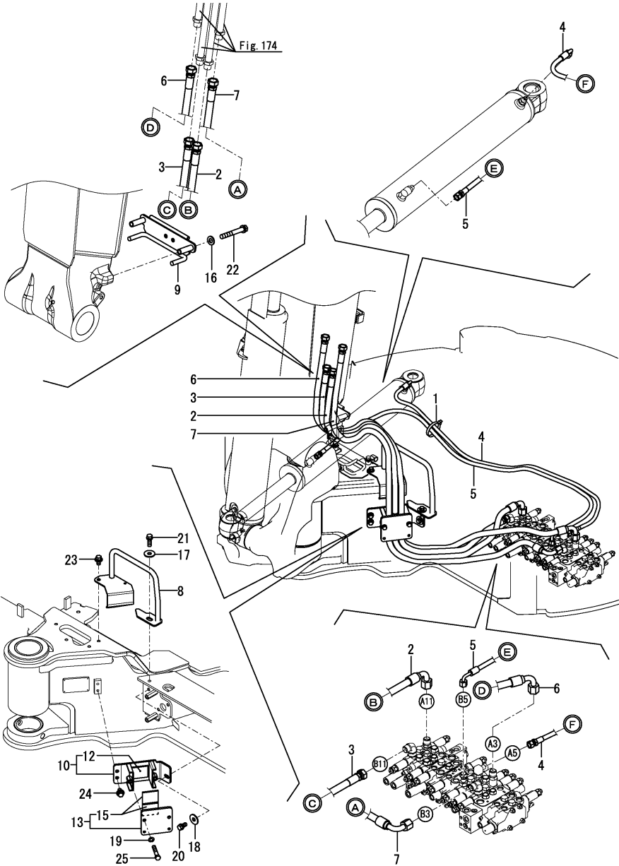
Fig.168. CONTROL VALVE - BOOM BULKHEAD & SWING
