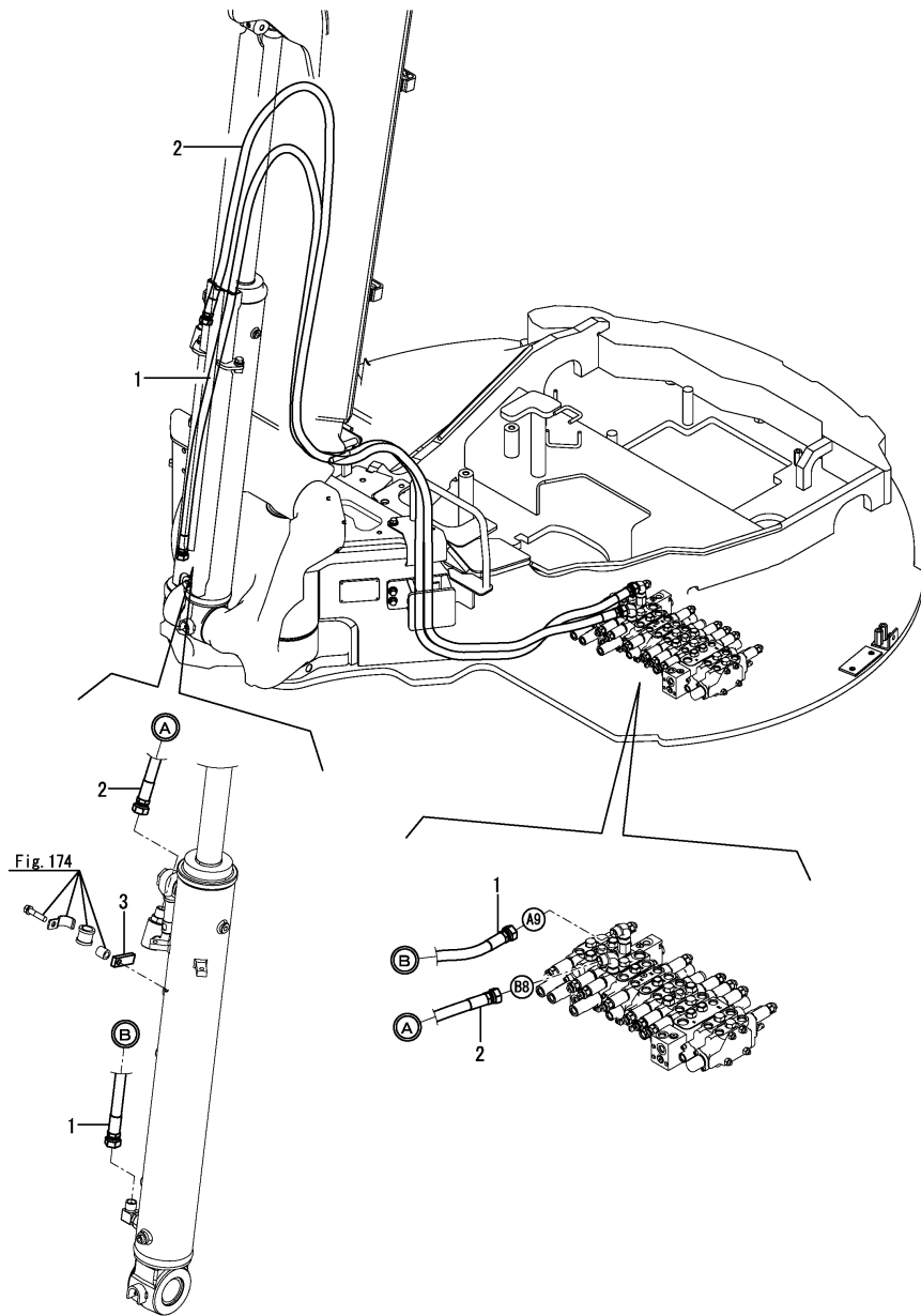
Fig.169. CONTROL VALVE - BOOM CYLINDER
