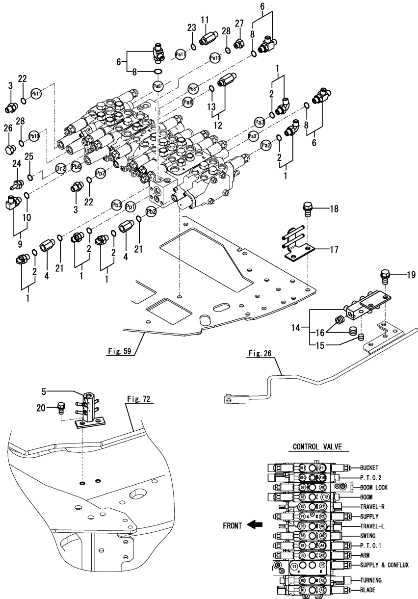
Fig.164. CONTROL VALVE(FITTING)(2)
