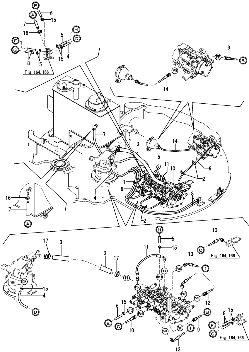
Fig.167. CONTROL VALVE - RETURN & DRAIN
