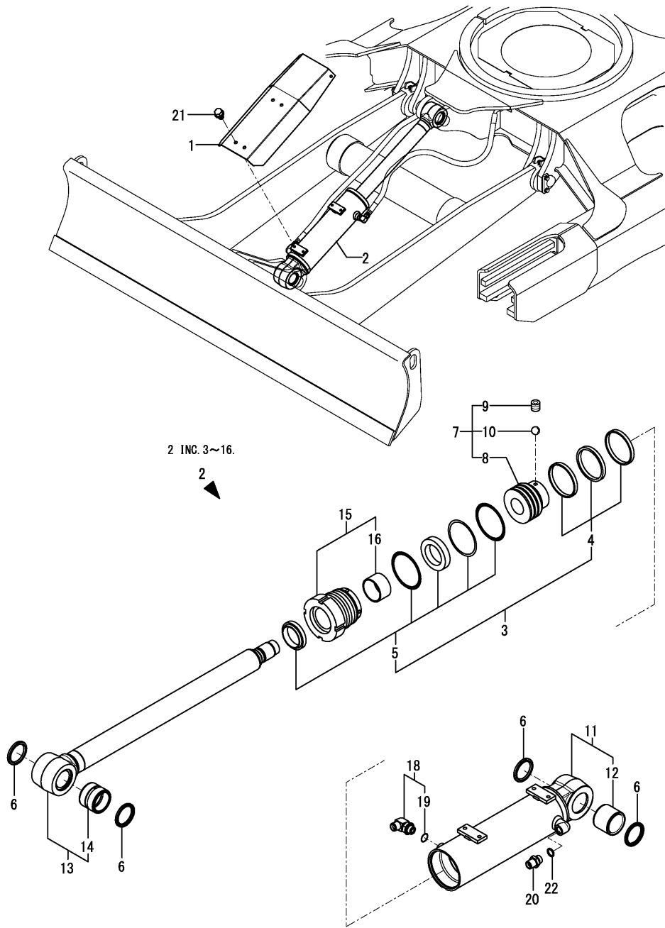
Fig.127. BLADE CYLINDER(QUICK COUPLER SPEC.)
