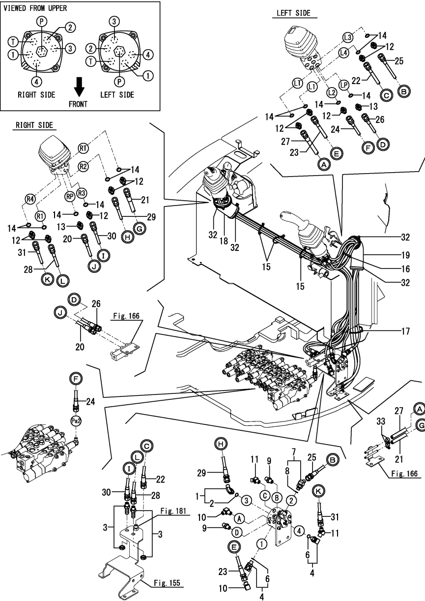
Fig.185. CONTROL PIPING(1)(ANGLE BLADE SPEC.)
