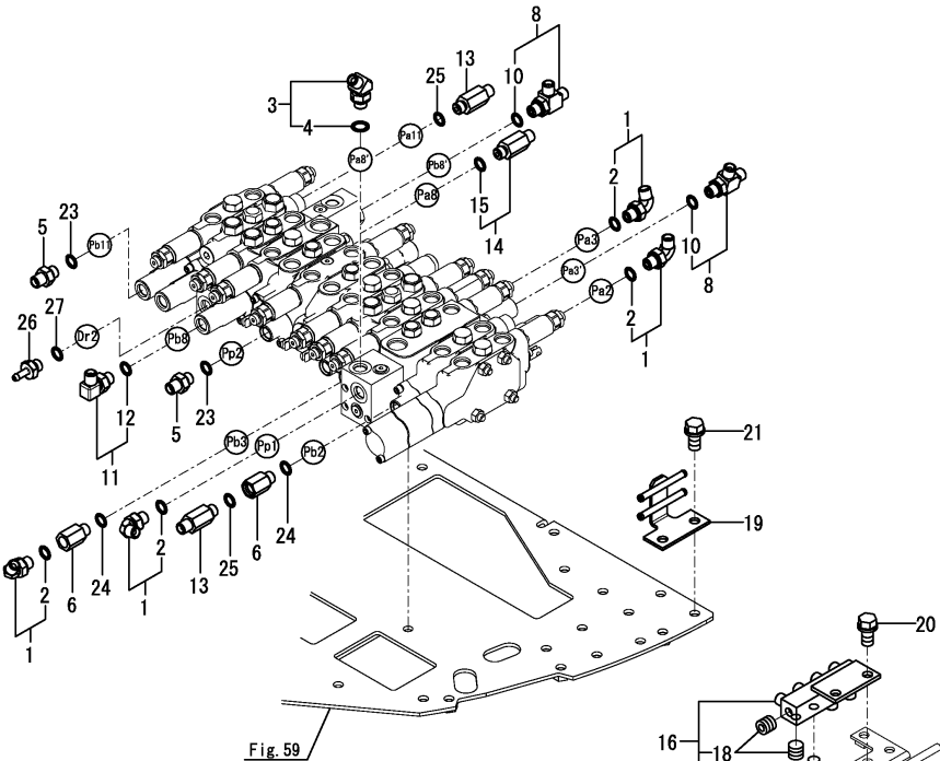
Fig.166. CONTROL VALVE(FITTING)(2)(ANGLE BLADE SPEC.)
