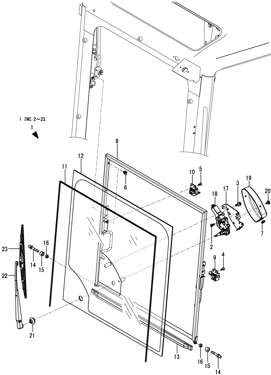
Fig.108. CABIN(FRONT WINDOW)(2)
