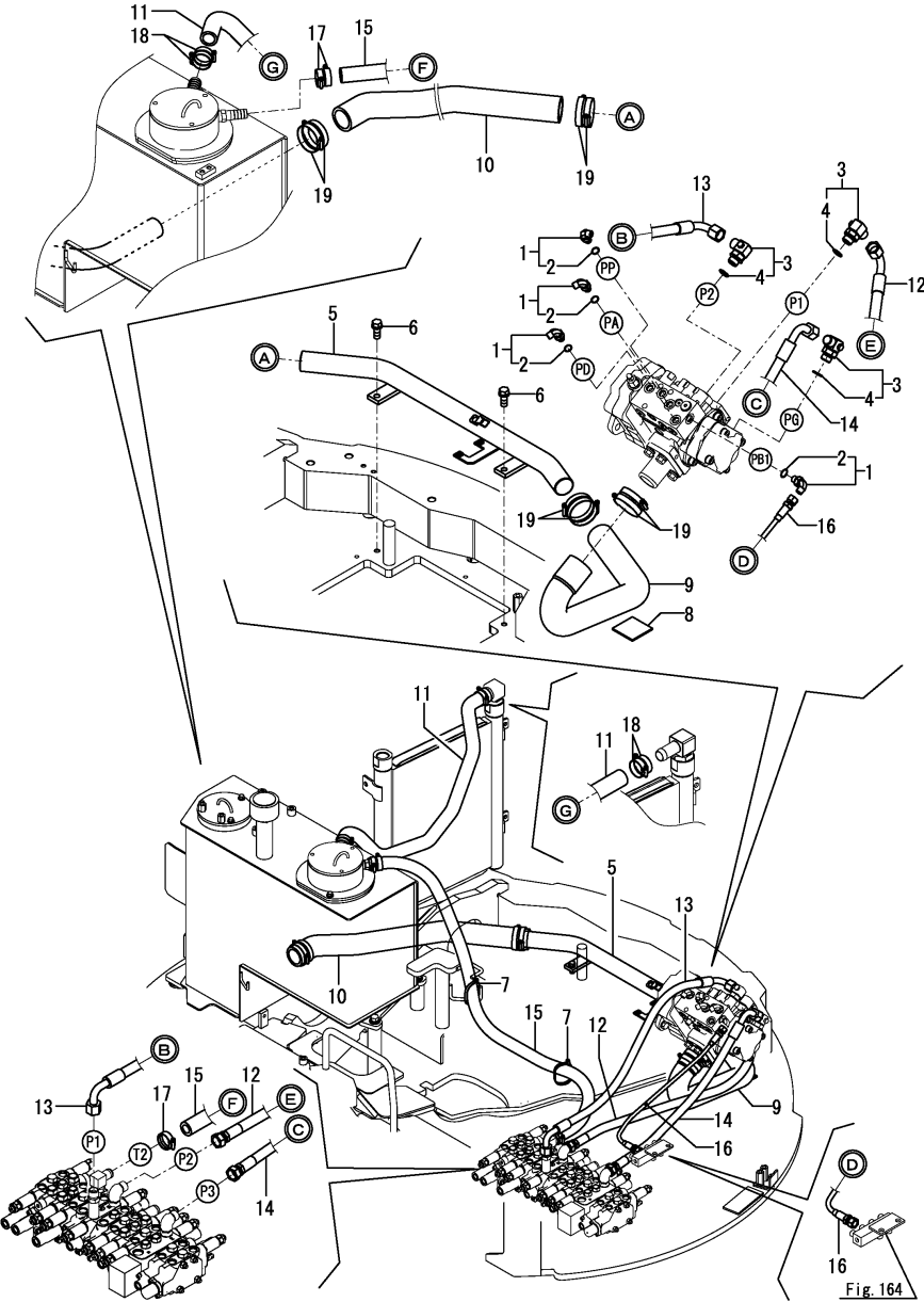
Fig.161. TANK - PUMP & CONTROL VALVE
