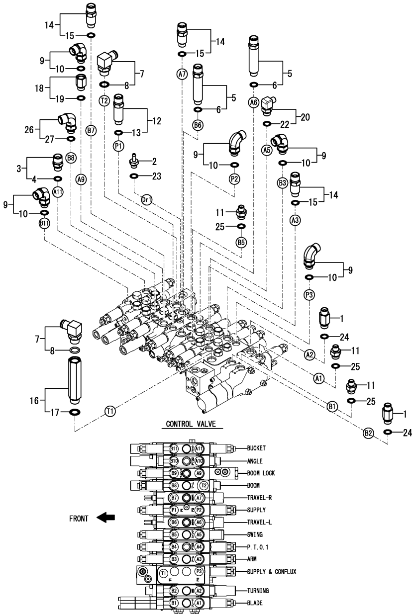
Fig.165. CONTROL VALVE(FITTING)(1)(ANGLE BLADE SPEC.)
