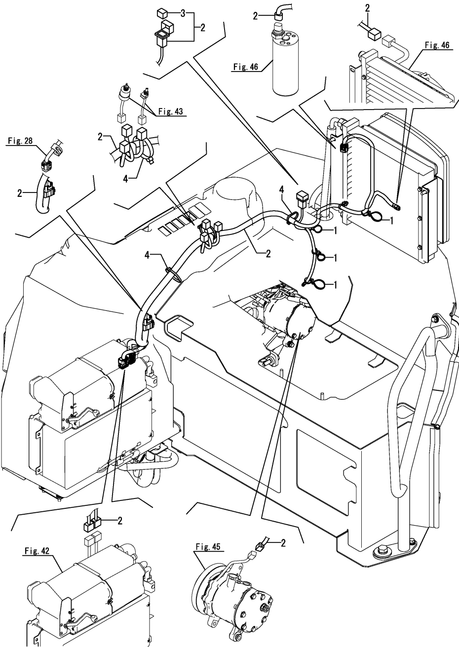
Fig.47. AIR CONDITIONER(ELECTRIC PARTS)
