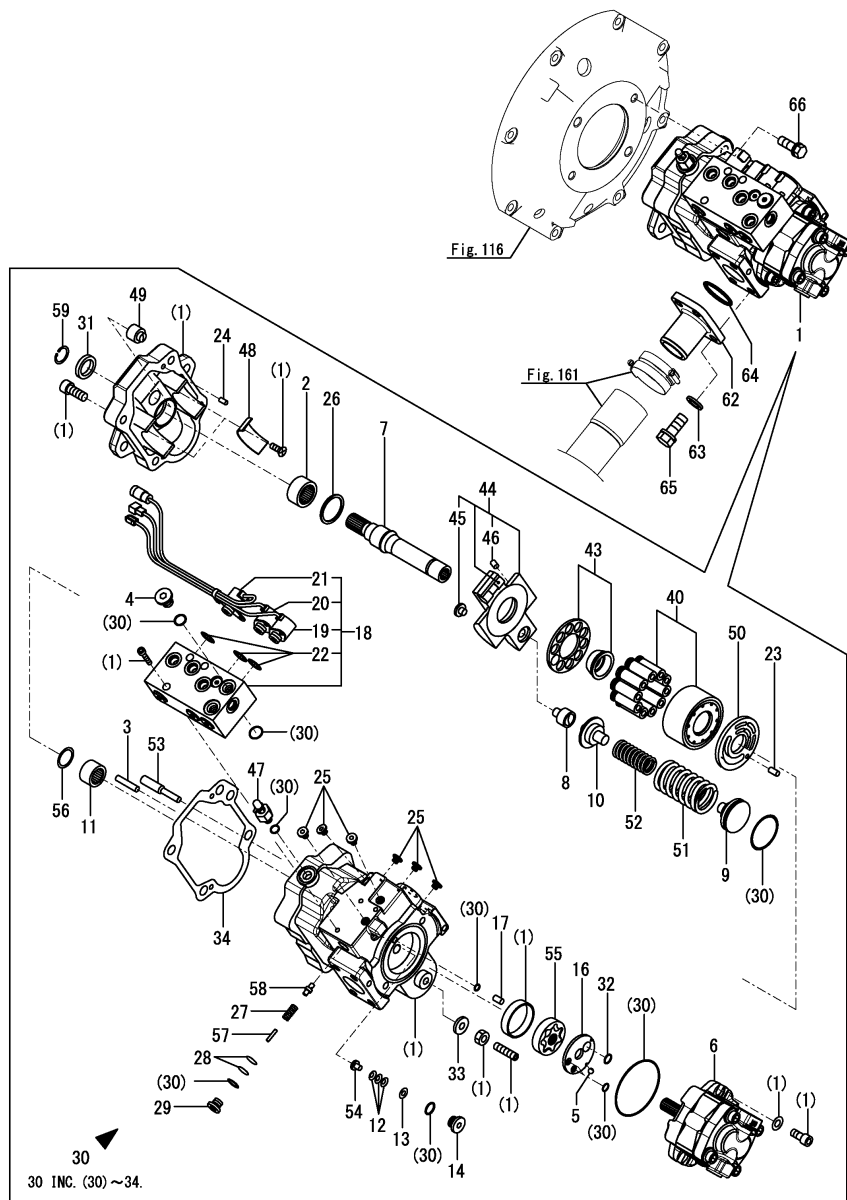
Fig.118. HYDRAULIC PUMP(QUICK COUPLER SPEC.)
