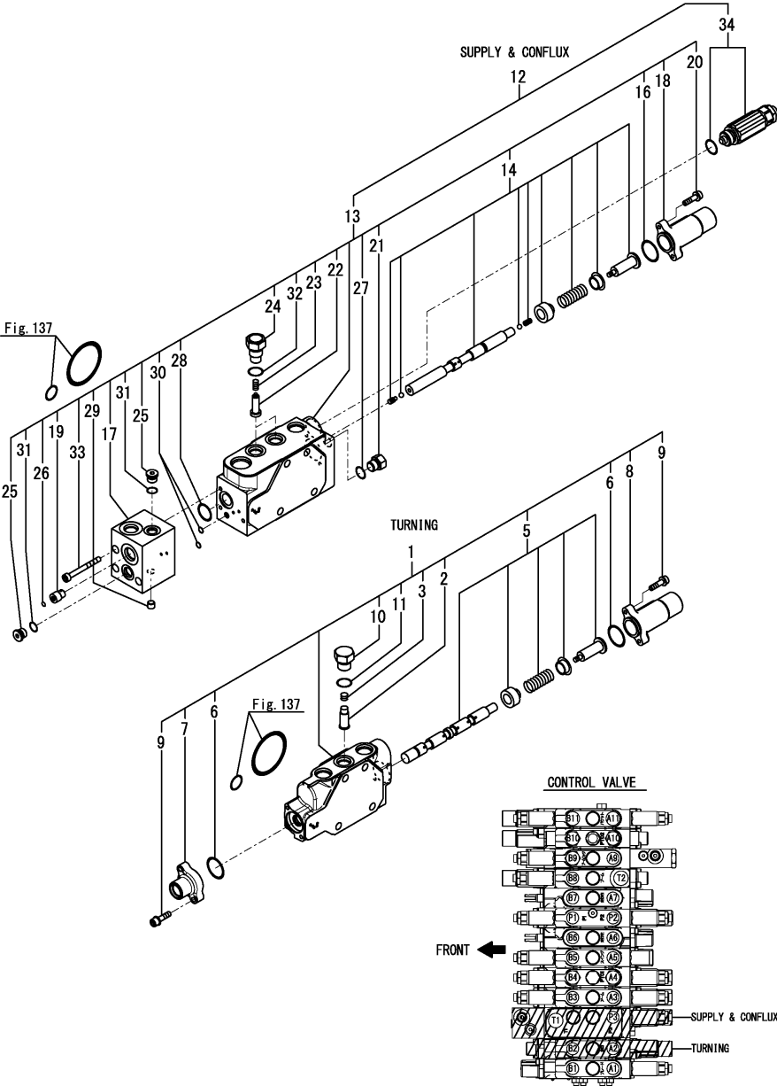
Fig.142. CONTROL VALVE(7/8)
