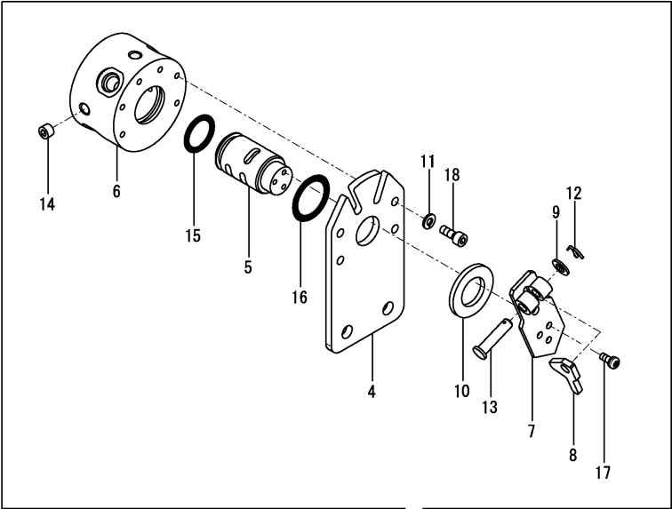
Fig.154. 2-WAY VALVE
